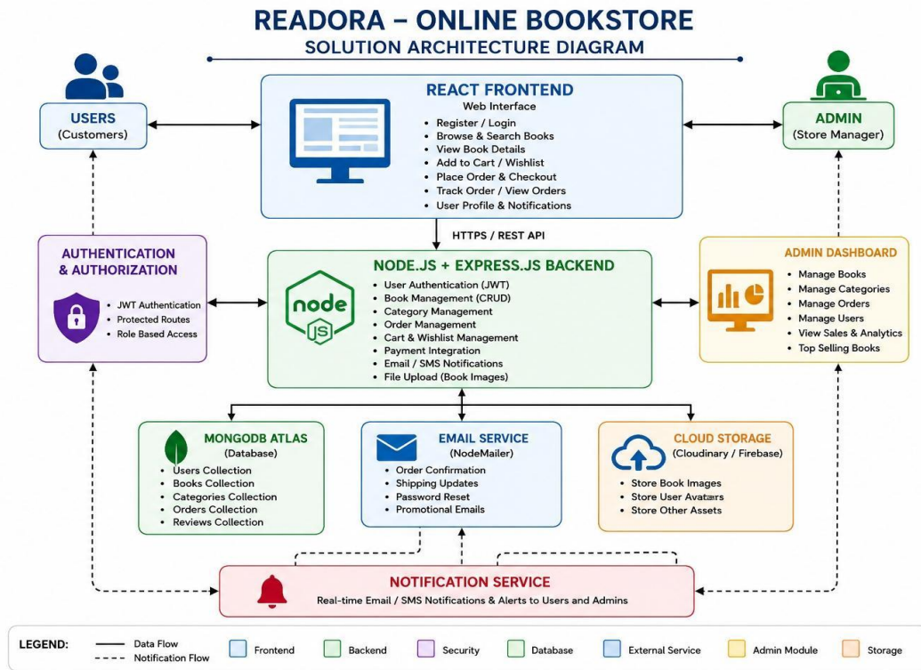
Figure 1: Architecture and data flow of the Readora-Bookstore.
